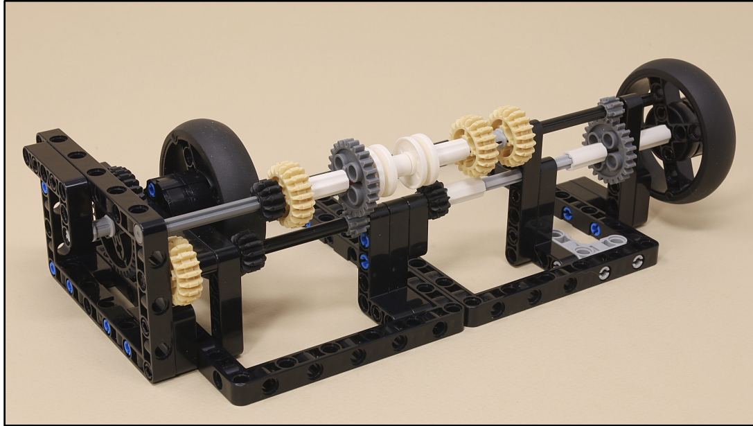
3-Speed Gearing
